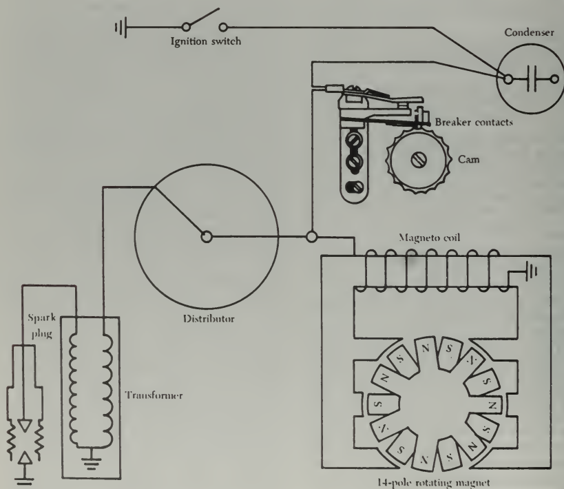
FIGURE 4-17. Low-tension system using a 14-pole rotating magnet.
